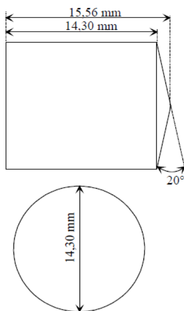
Figure 17.14.1: Standard fragment for 1.6 article fragment impact test
